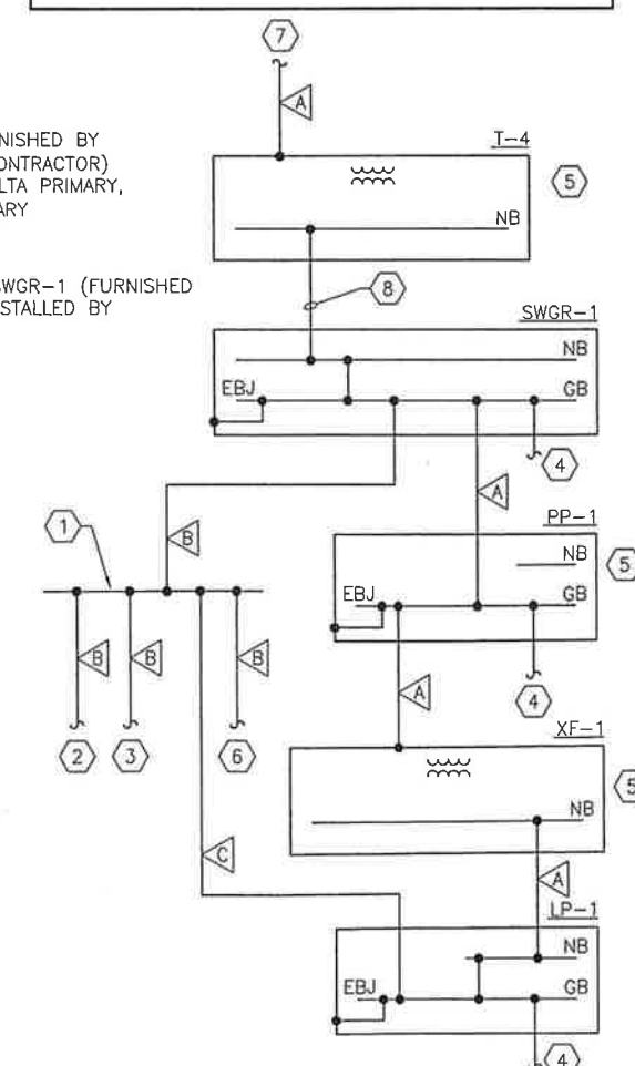
3 GROUNDING ONE-LINE DIAGRAM NO SCALE
