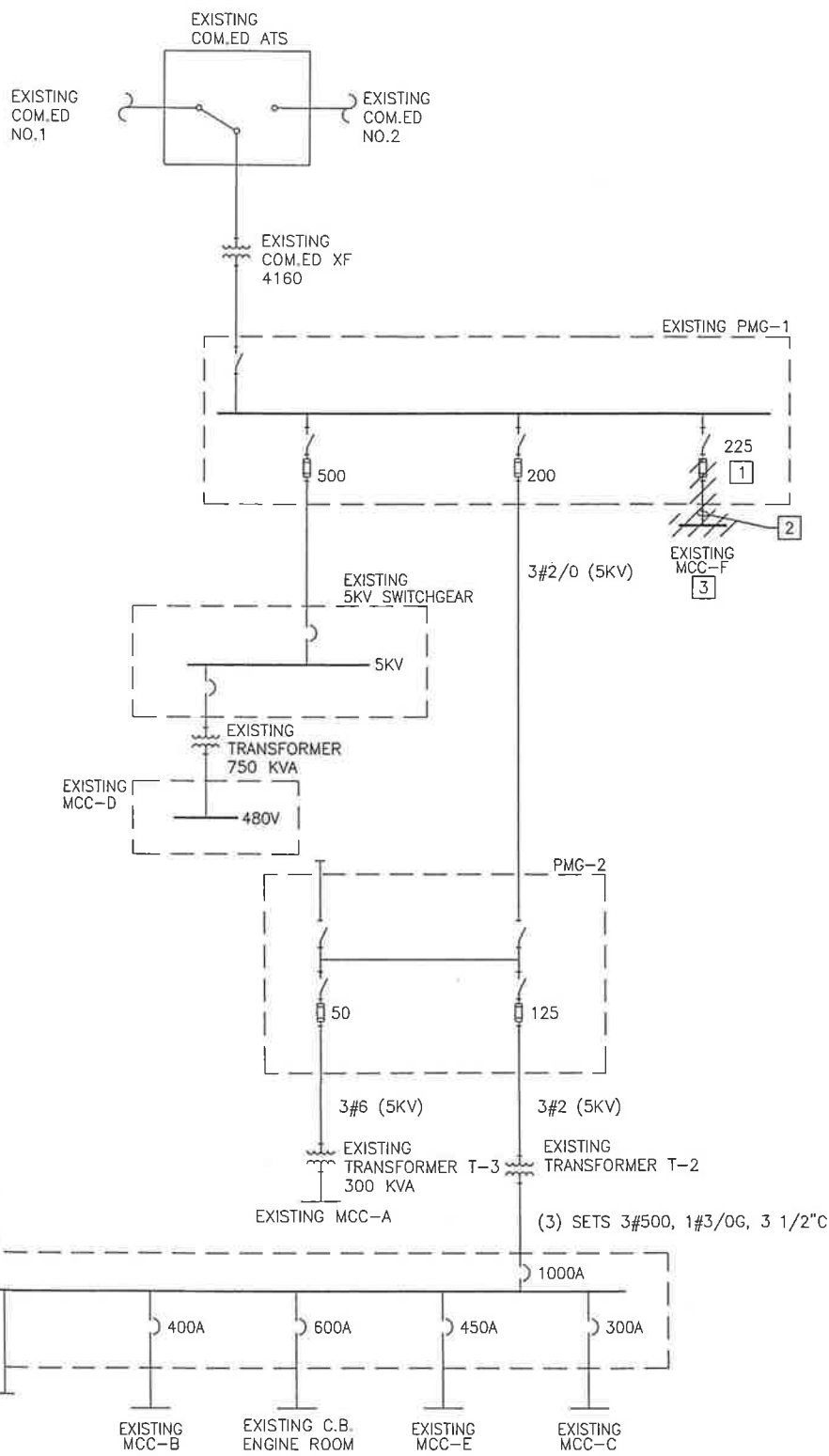
1 DEMOLITION POWER ONE-LINE DIAGRAM NO SCALE
